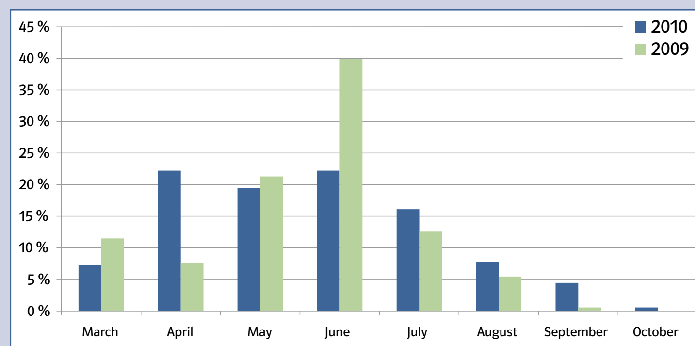
Fig. 1: Relative occurrence of the day with the maximal feed in power of 150 distributed PV systems in Bavaria.
