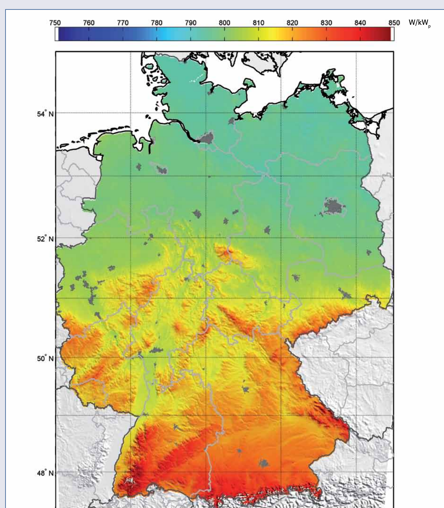
Fig. 3: The maximal feed in power of a typical south oriented PV system for Germany appearing in June in W/kW p installed STC power.
