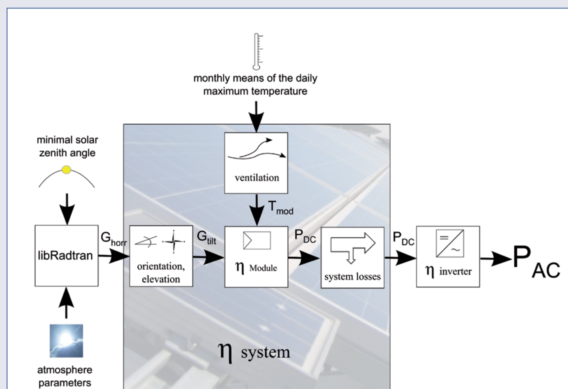
Fig. 2: Block diagram of the simulation model.
